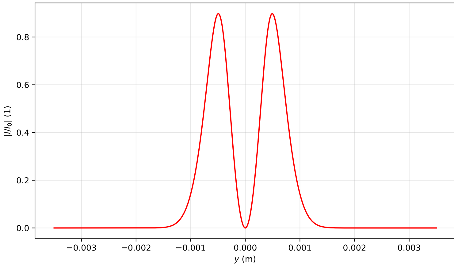
Intensity profile I(x=0, y, z=0.159)/I_0 , P_{in}=6.0P_{cr} , artificial time
